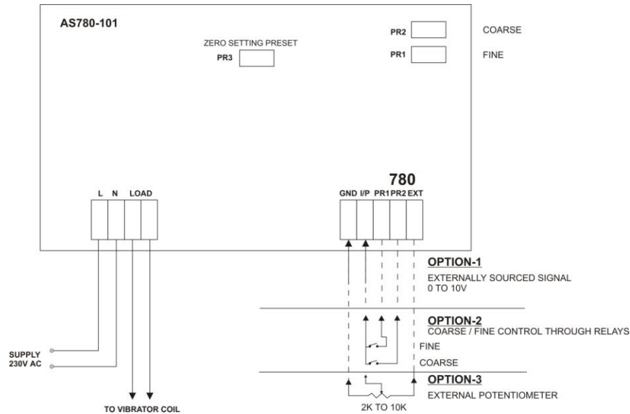
Wiring diagram
