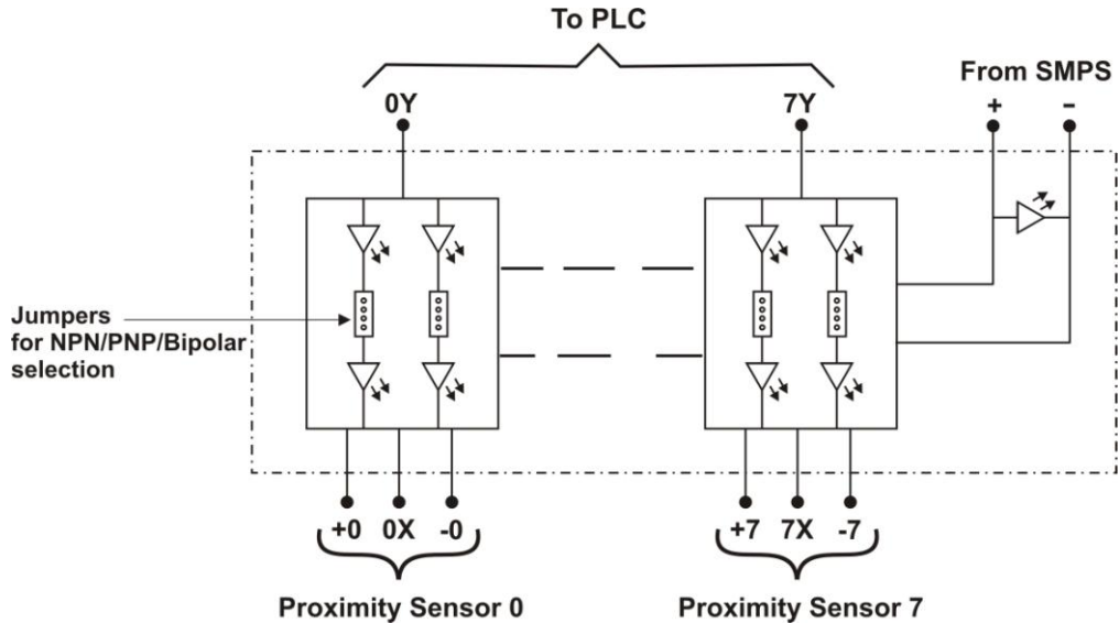
Wiring Diagram
