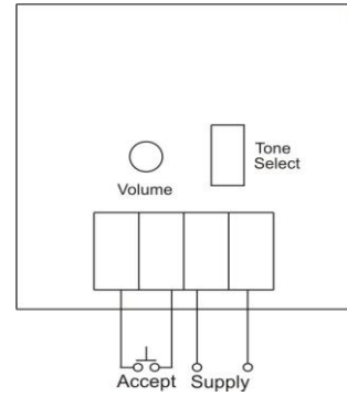
Terminal Connection
