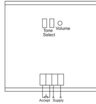
Terminal Connection
